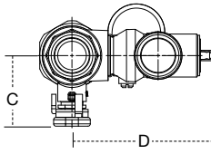
3/4" LFTWH-FT/FS-H-RV
